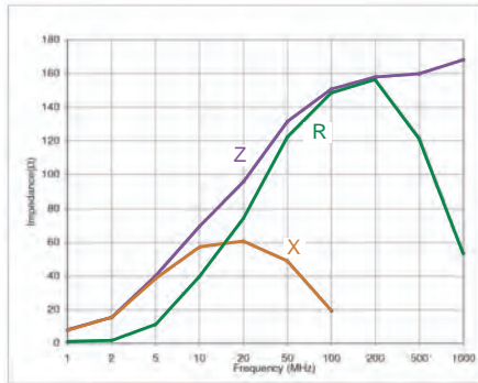
Z-f Charecteristics
